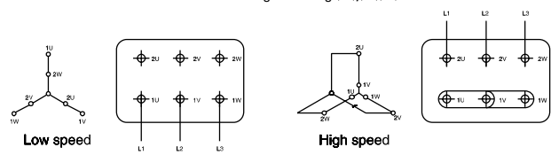
Single winding \Delta/\Delta
