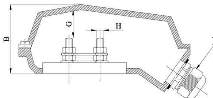
VIEW W/O TERMINAL BOX COVER
